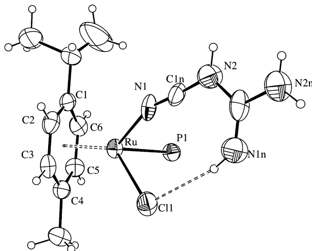
Figure 1. ORTEP view of the cation of 1b . The ethoxy and phenyl groups of the phosphonite group are not drawn. The atoms are drawn at the 30% probability level.
