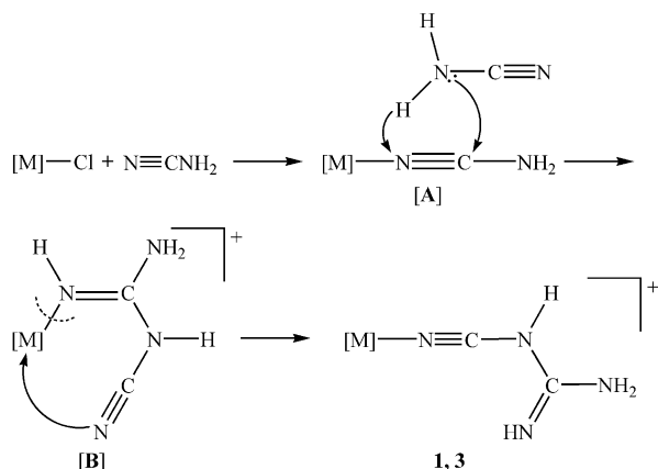
Scheme 2. [M] = [MCl(\eta^6\text{-}p\text{-cymene})(PR_3)] .
