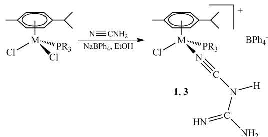
Scheme 1. \text{M} = \text{Ru} ( 1 ), \text{Os} ( 3 ); \text{PR}_3 = \text{P}(\text{OEt})_3 ( a ), \text{PPh}(\text{OEt})_2 ( b ), \text{PPh}_2\text{OEt} ( c ), \text{PiPr}_3 ( d ).
