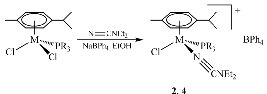
Scheme 3. M = Ru ( 2 ), Os ( 4 ); PR_3 = PPh(OEt)_2 ( b ).
