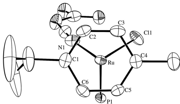
Figure 2. ORTEP drawn of the cation view along the Ct–Ru vector.
